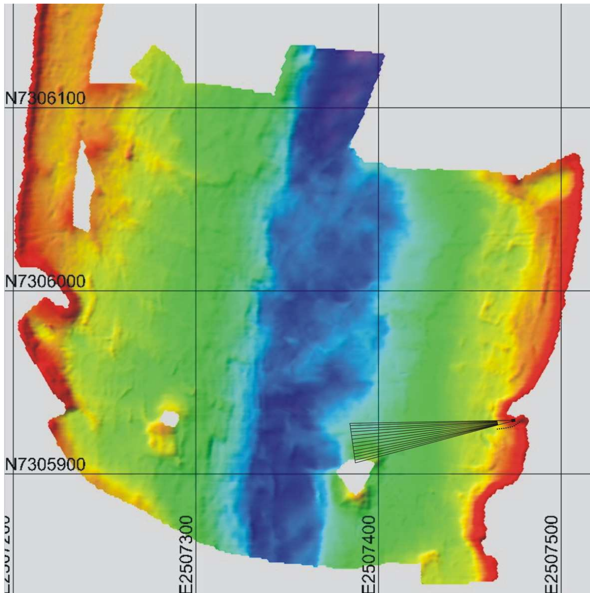
Figure 2. A bottom map of the Tornio site. The DIDSON sonar on the east shore and the beam coverage. Blue colour describes the deepest and red the shallowest area of the river. Finnish national coordinates with 100 × 100 m grid lines.
