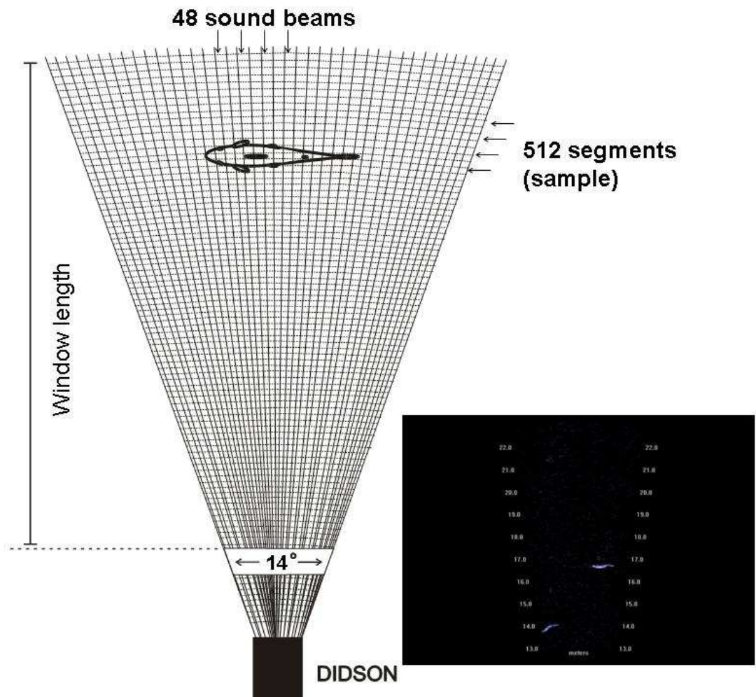
Figure 5. A schematic picture (from above) of a DIDSON frame (image) and a snapshot of the DIDSON screen where two salmon were swimming from right to left.
